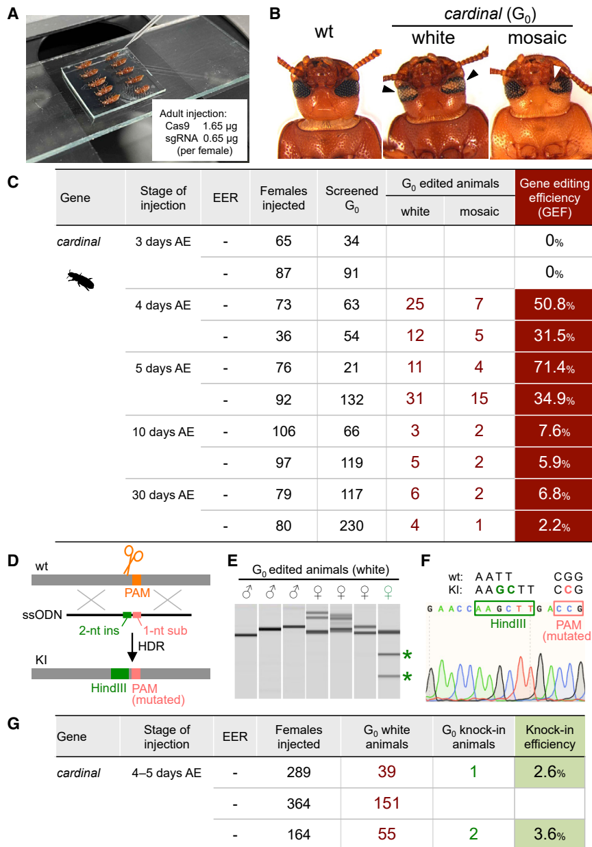
Figure 3. DIPA-CRISPR in beetles
